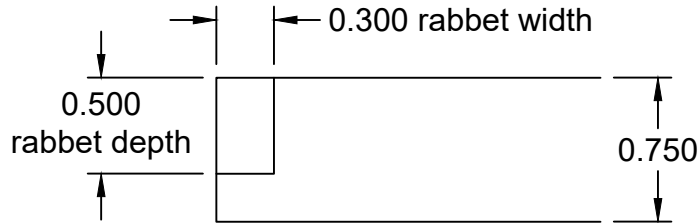
RABBET DETAIL
